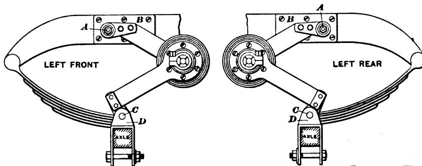
TRUFFAULT-HARTFORD SUSPENSION DEVICE ATTACHED AT FRONT AND REAR OF FRAME.
